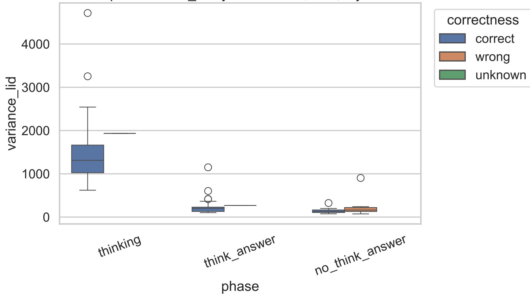
Exp C variance_lid by correctness, 32B, layer 6
