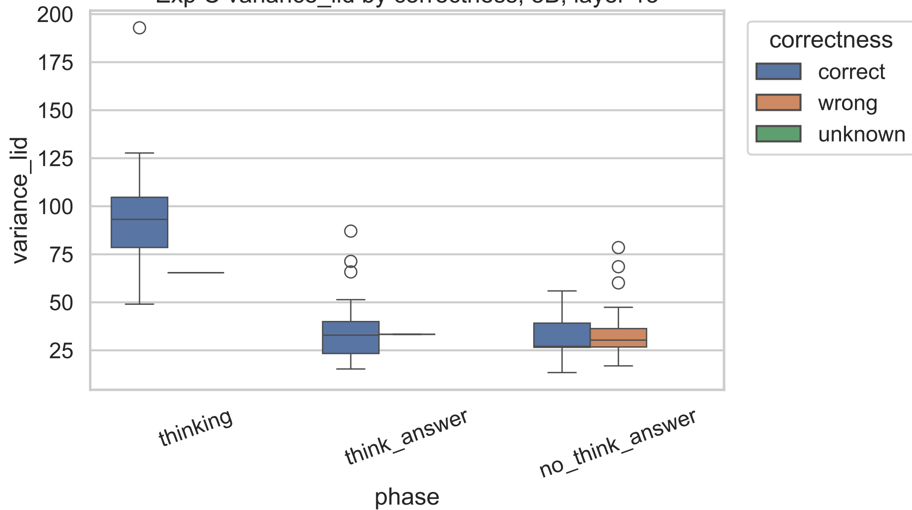
Exp C variance_lid by correctness, 8B, layer 13
