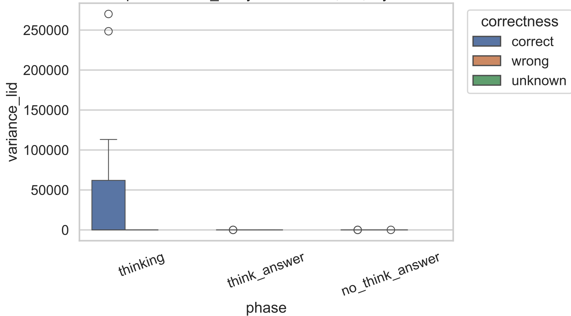
Exp C variance_lid by correctness, 8B, layer 20
