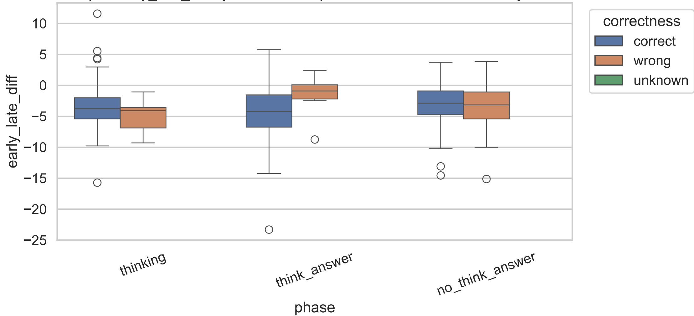
Exp C early_late_diff by correctness, pooled across model sizes, layer 13
