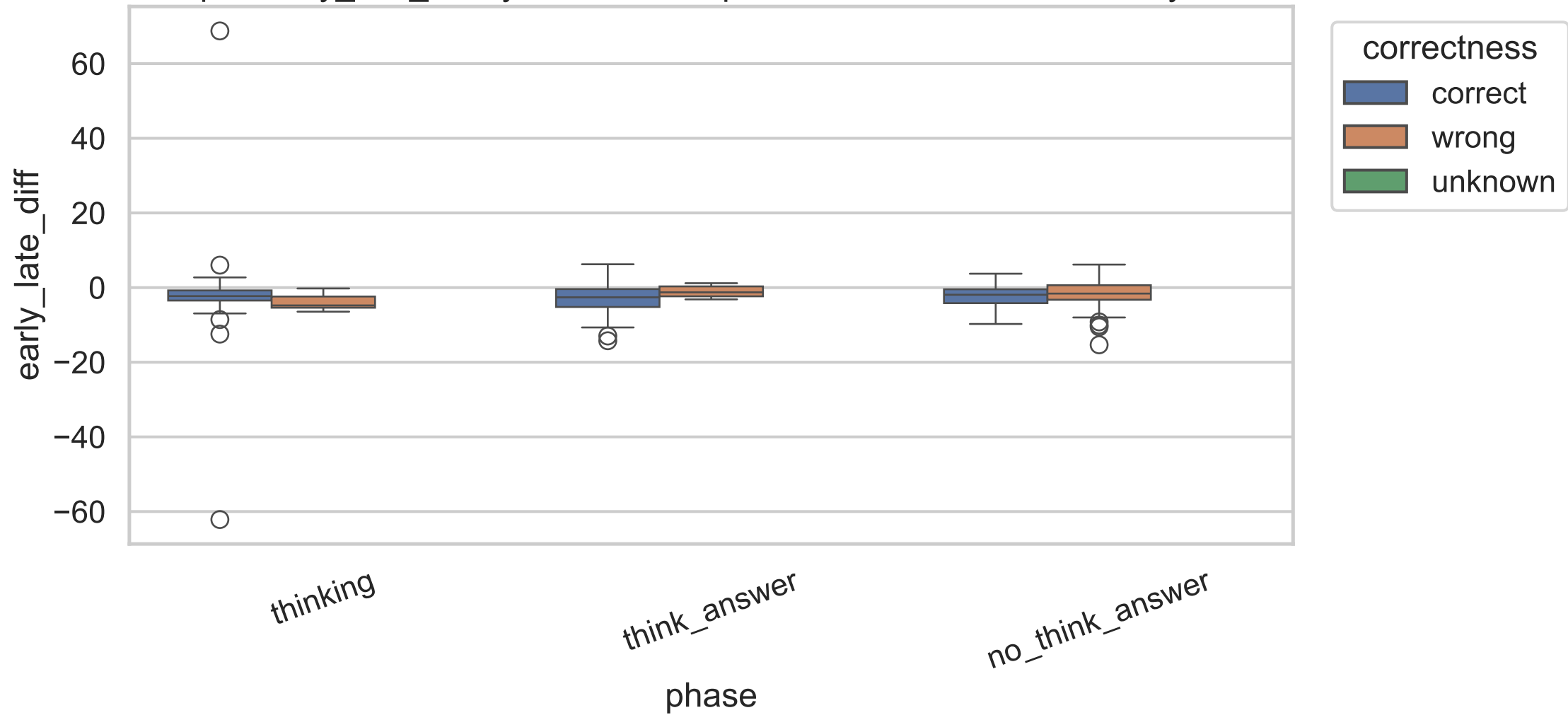
Exp C early_late_diff by correctness, pooled across model sizes, layer 20
