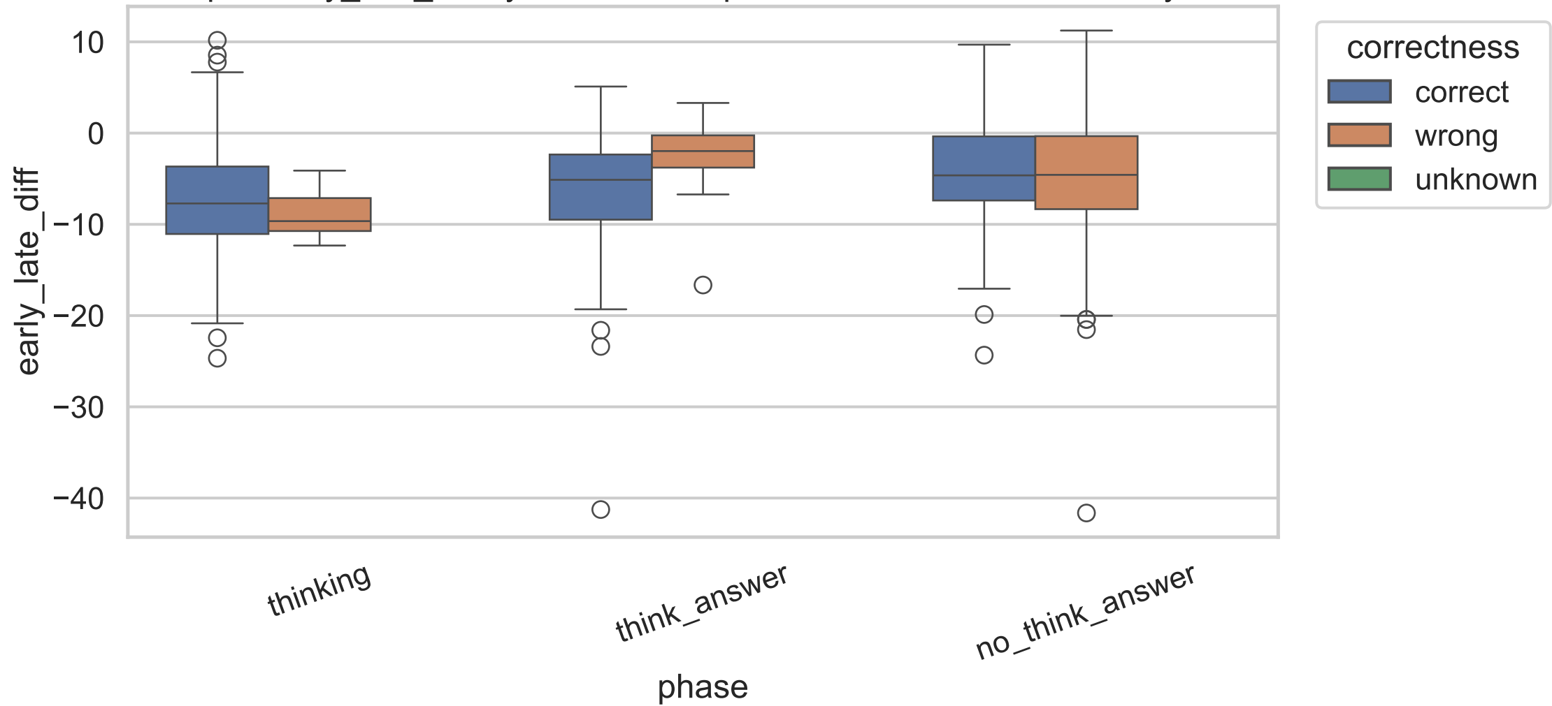
Exp C early_late_diff by correctness, pooled across model sizes, layer 6
