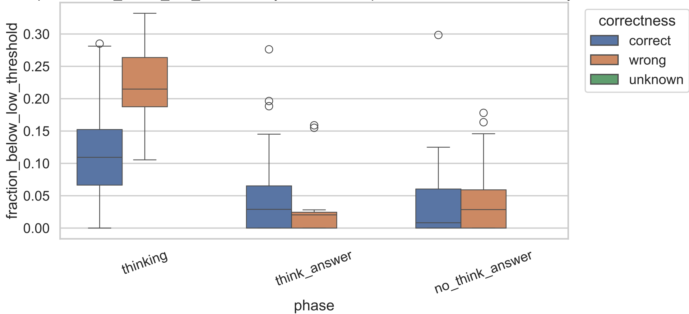
Exp C fraction_below_low_threshold by correctness, pooled across model sizes, layer 13
