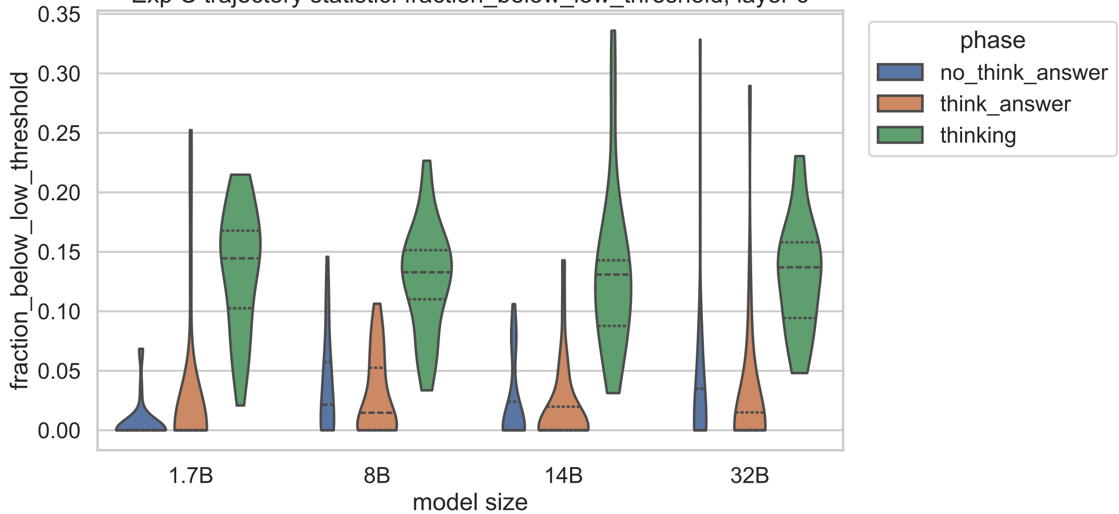
Exp C trajectory statistic: fraction_below_low_threshold, layer 6
