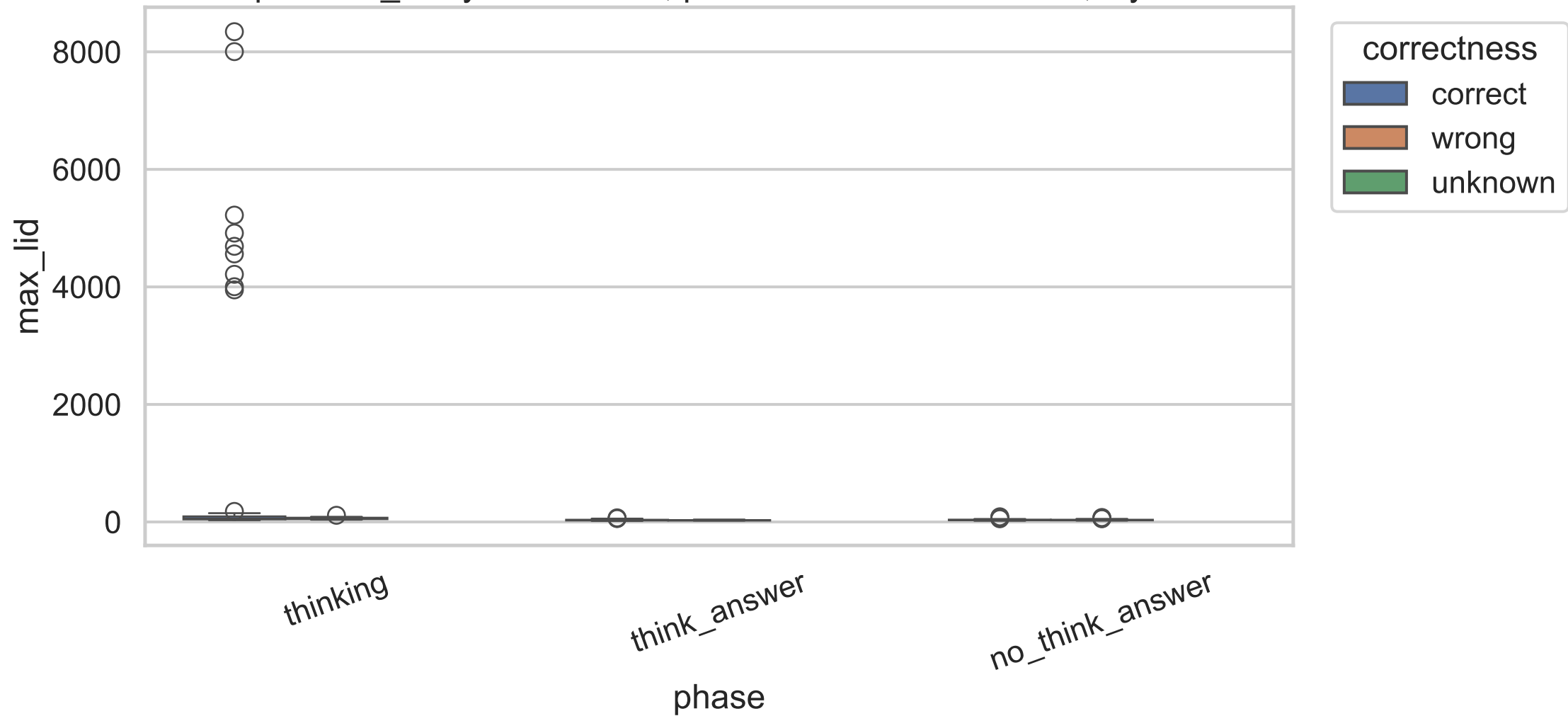
Exp C max_lid by correctness, pooled across model sizes, layer 20
