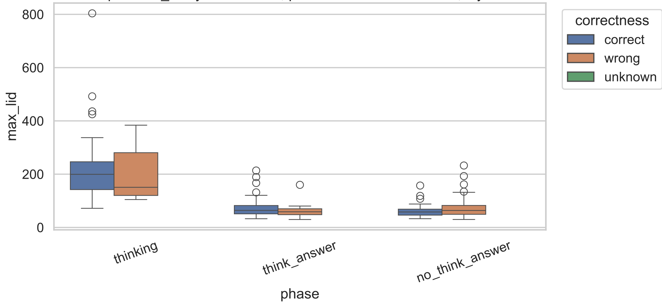
Exp C max_lid by correctness, pooled across model sizes, layer 6
