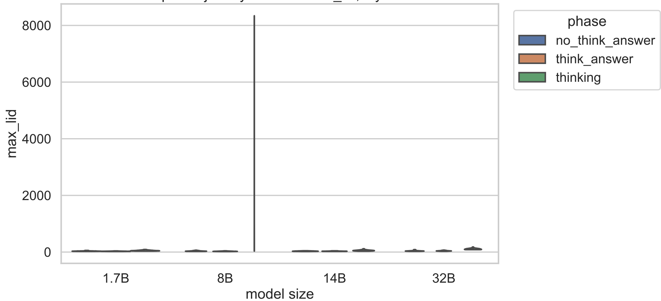
Exp C trajectory statistic: max_lid, layer 20
