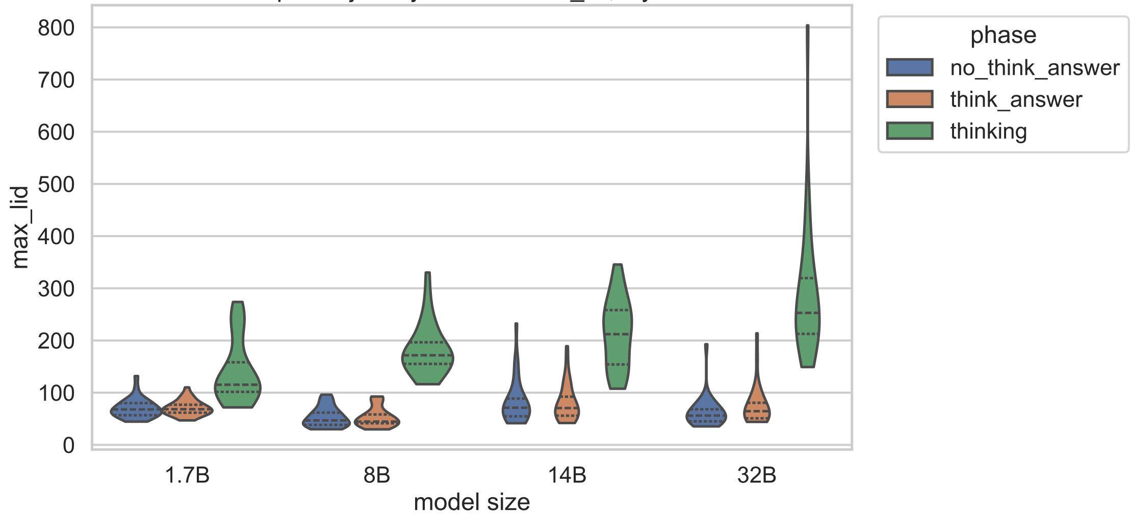
Exp C trajectory statistic: max_lid, layer 6
