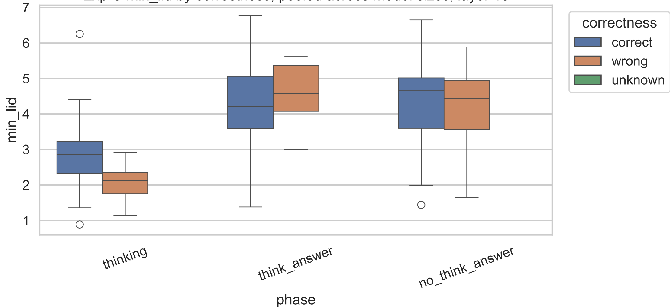
Exp C min_lid by correctness, pooled across model sizes, layer 13
