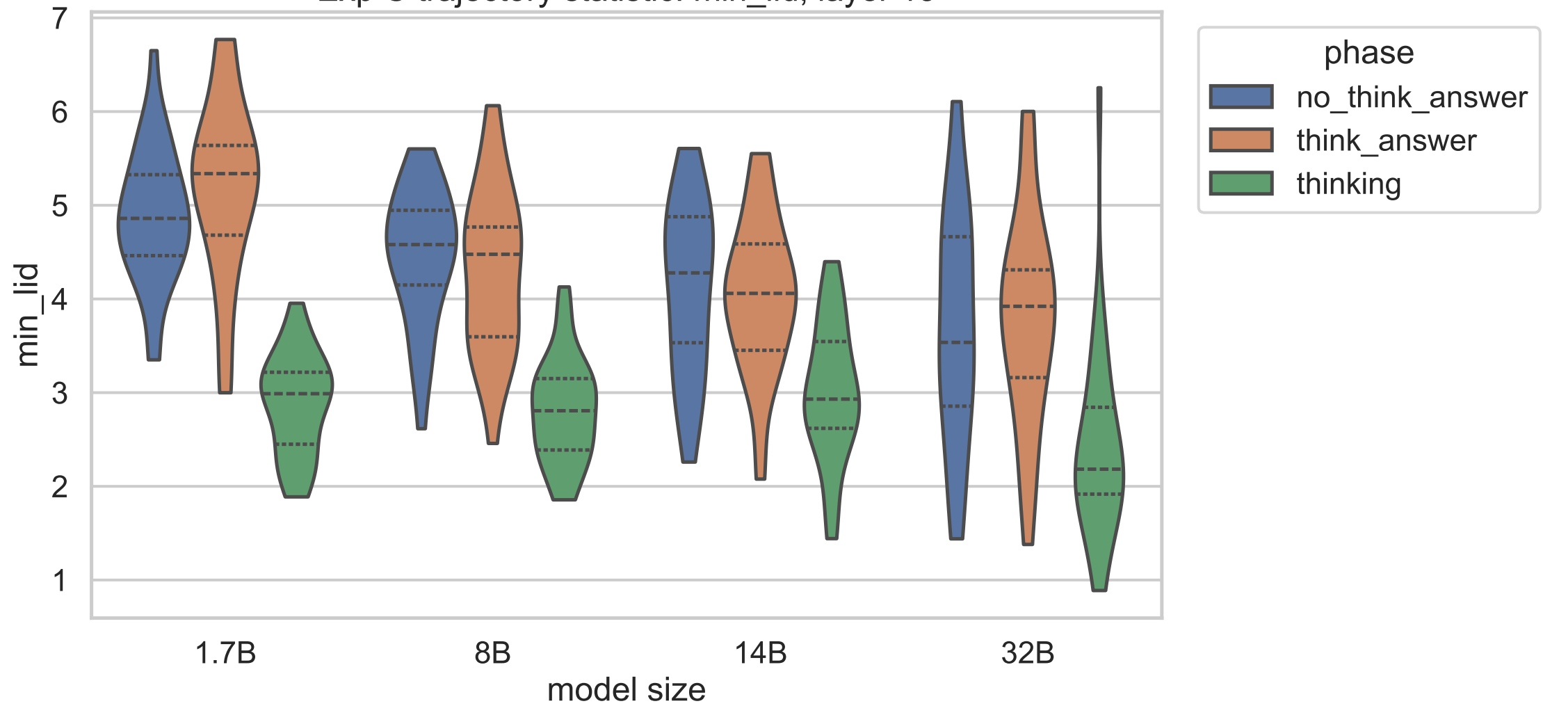
Exp C trajectory statistic: min_lid, layer 13
