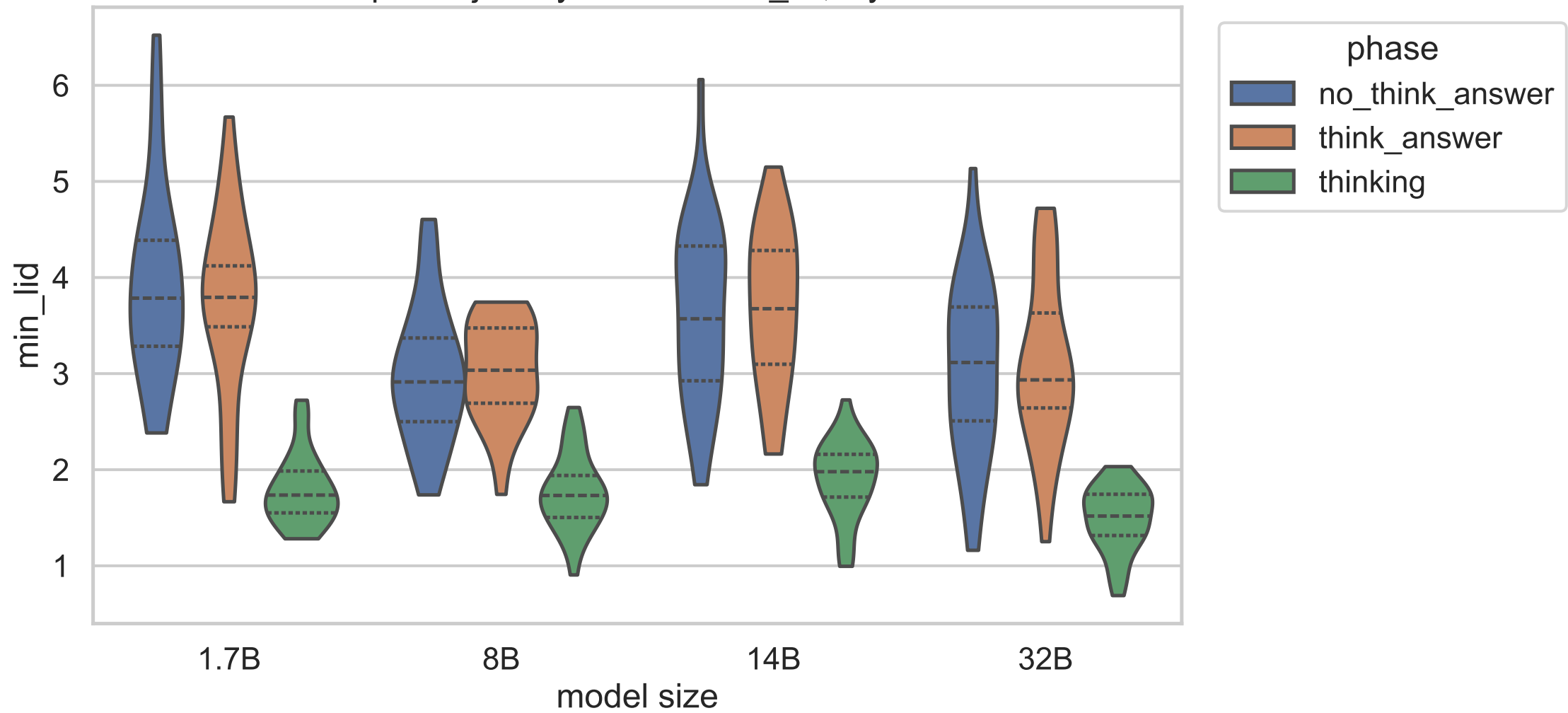
Exp C trajectory statistic: min_lid, layer 6
