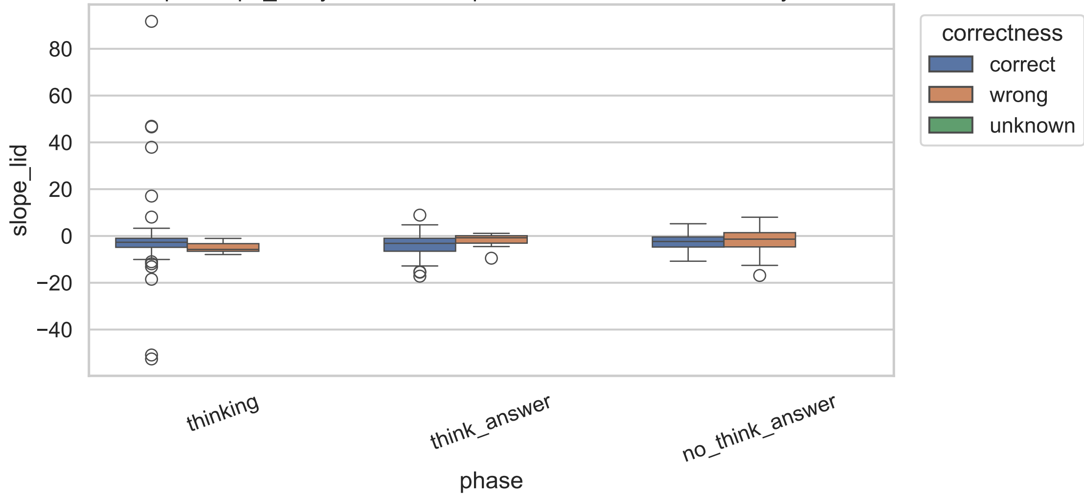
Exp C slope_lid by correctness, pooled across model sizes, layer 20
