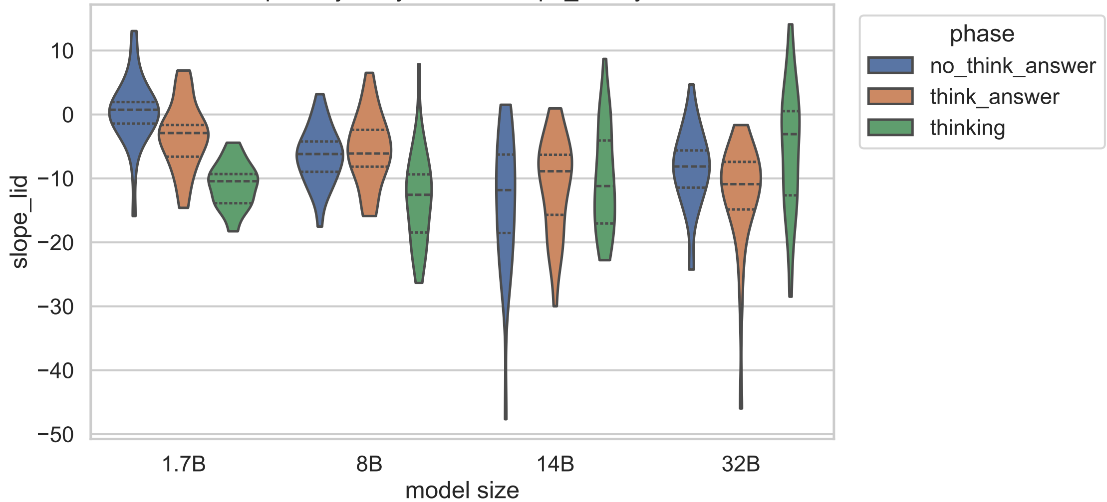
Exp C trajectory statistic: slope_lid, layer 6
