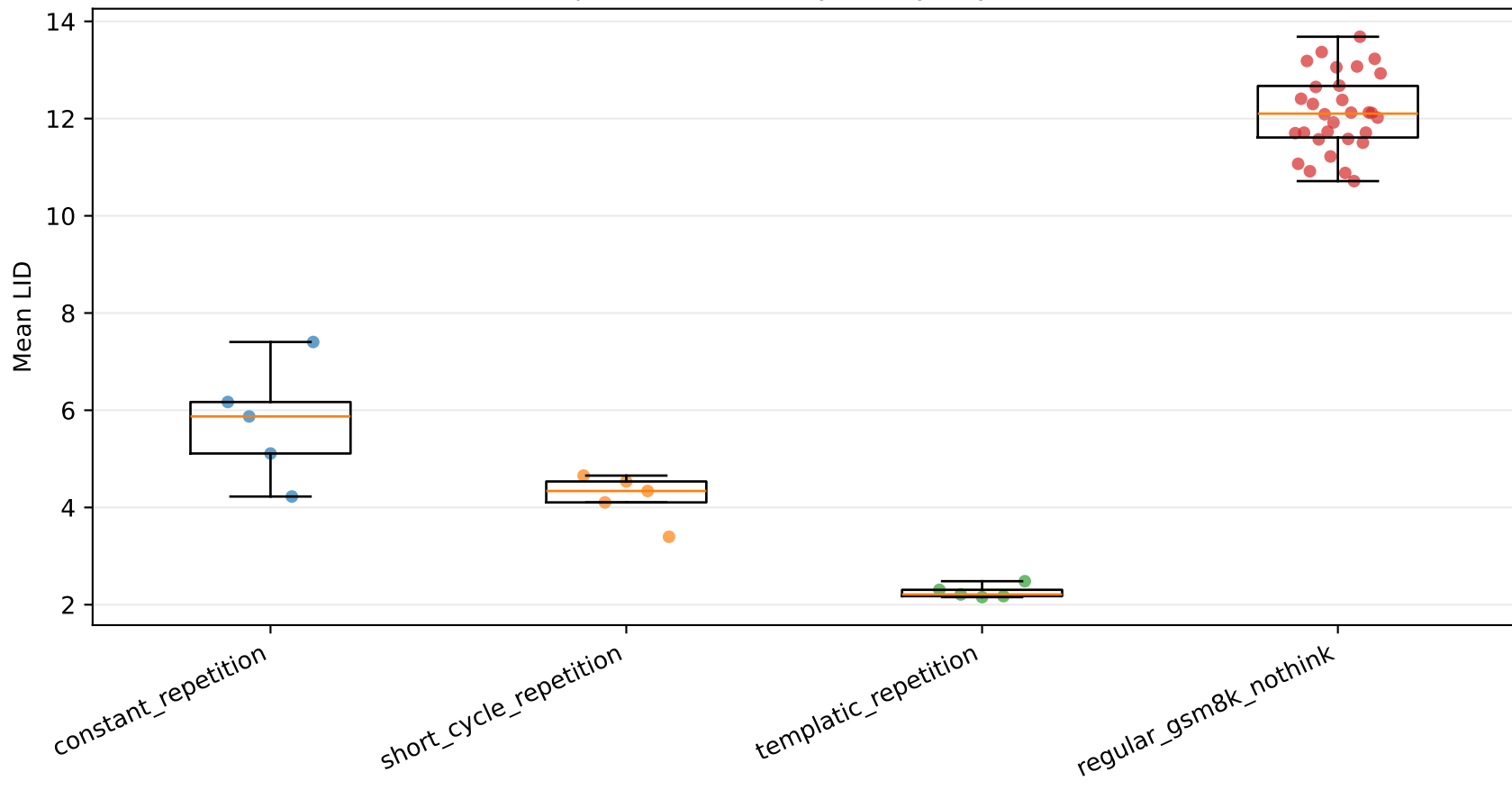
Experiment A LID by family, layer 13
