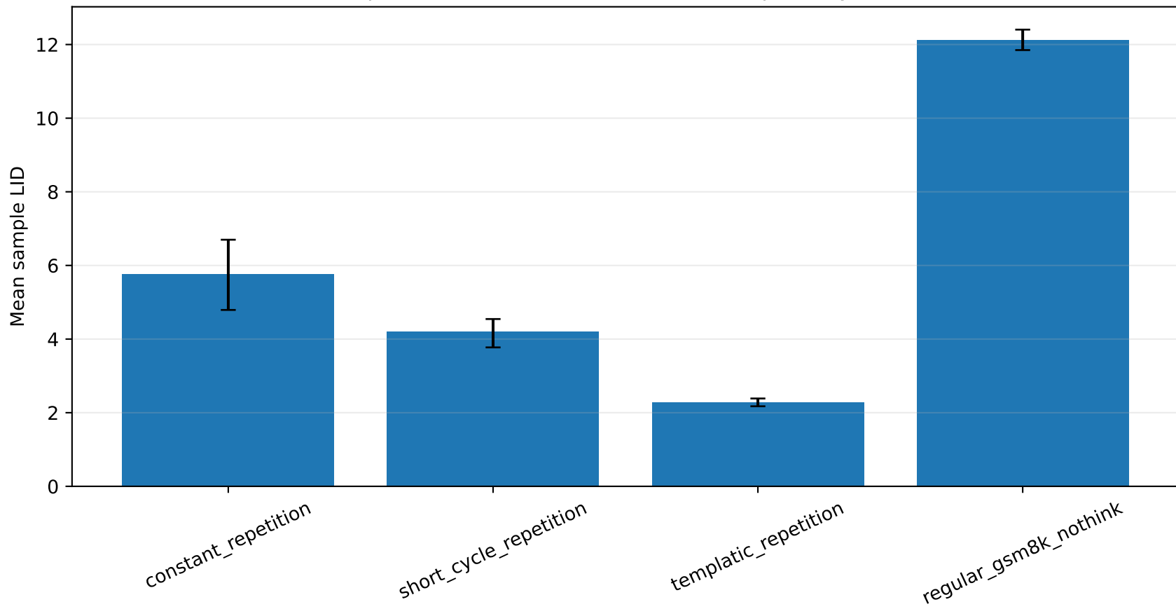
Experiment A mean LID with bootstrap CI, layer 13
