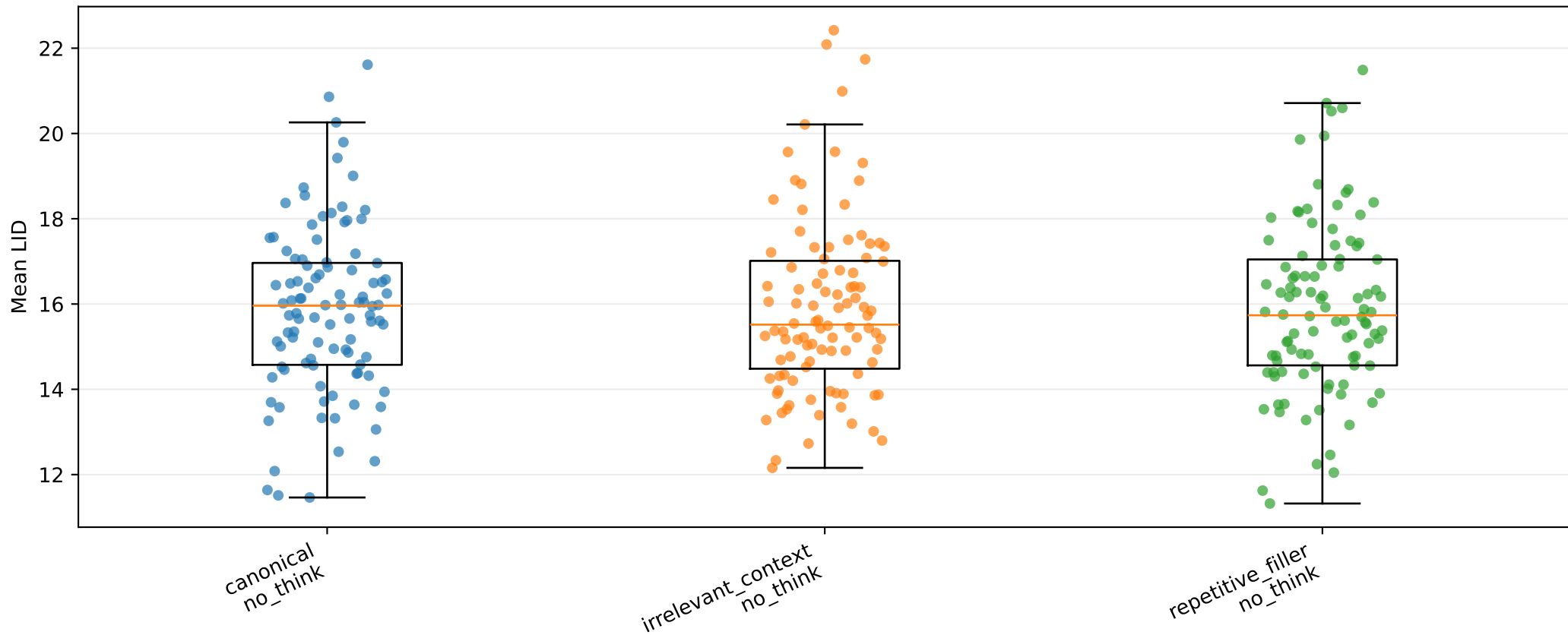
Experiment B answer LID, layer 6
