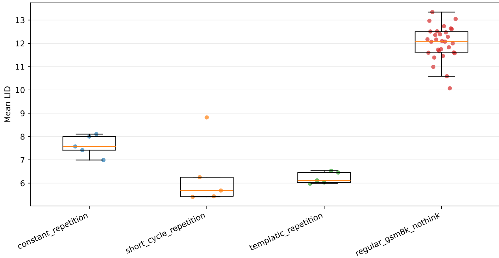
Experiment A LID by family, layer 20
