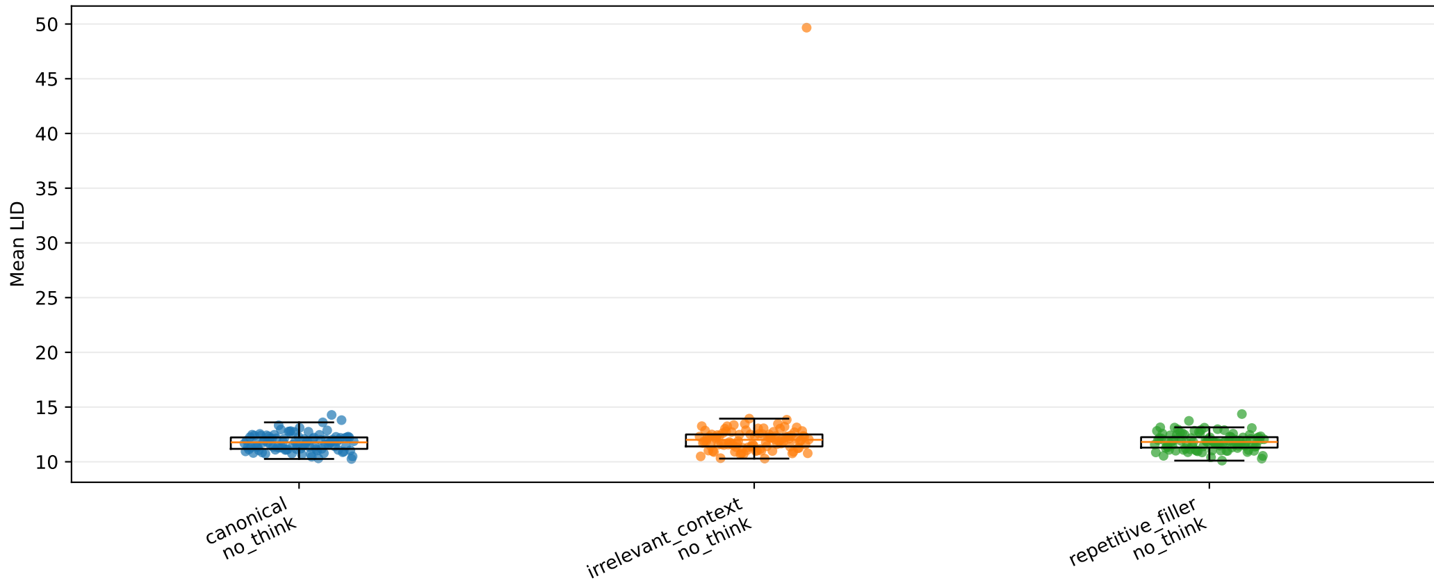
Experiment B answer LID, layer 20
