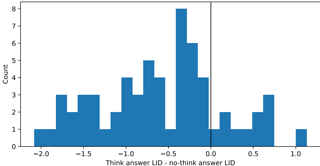
Experiment C paired differences, layer 20
