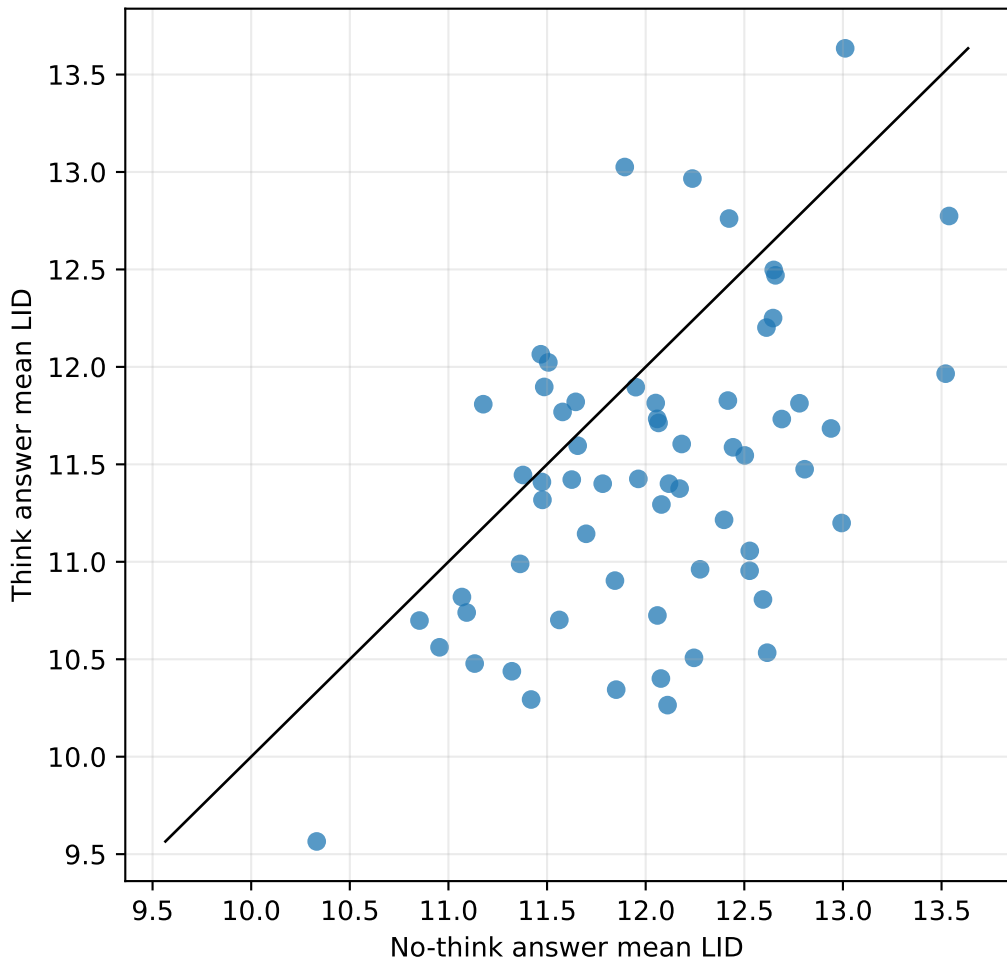
Experiment C paired answer LID, layer 20
