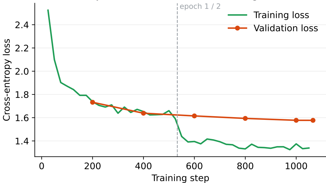
NaijaReviewer-8B QLoRA fine-tuning loss
