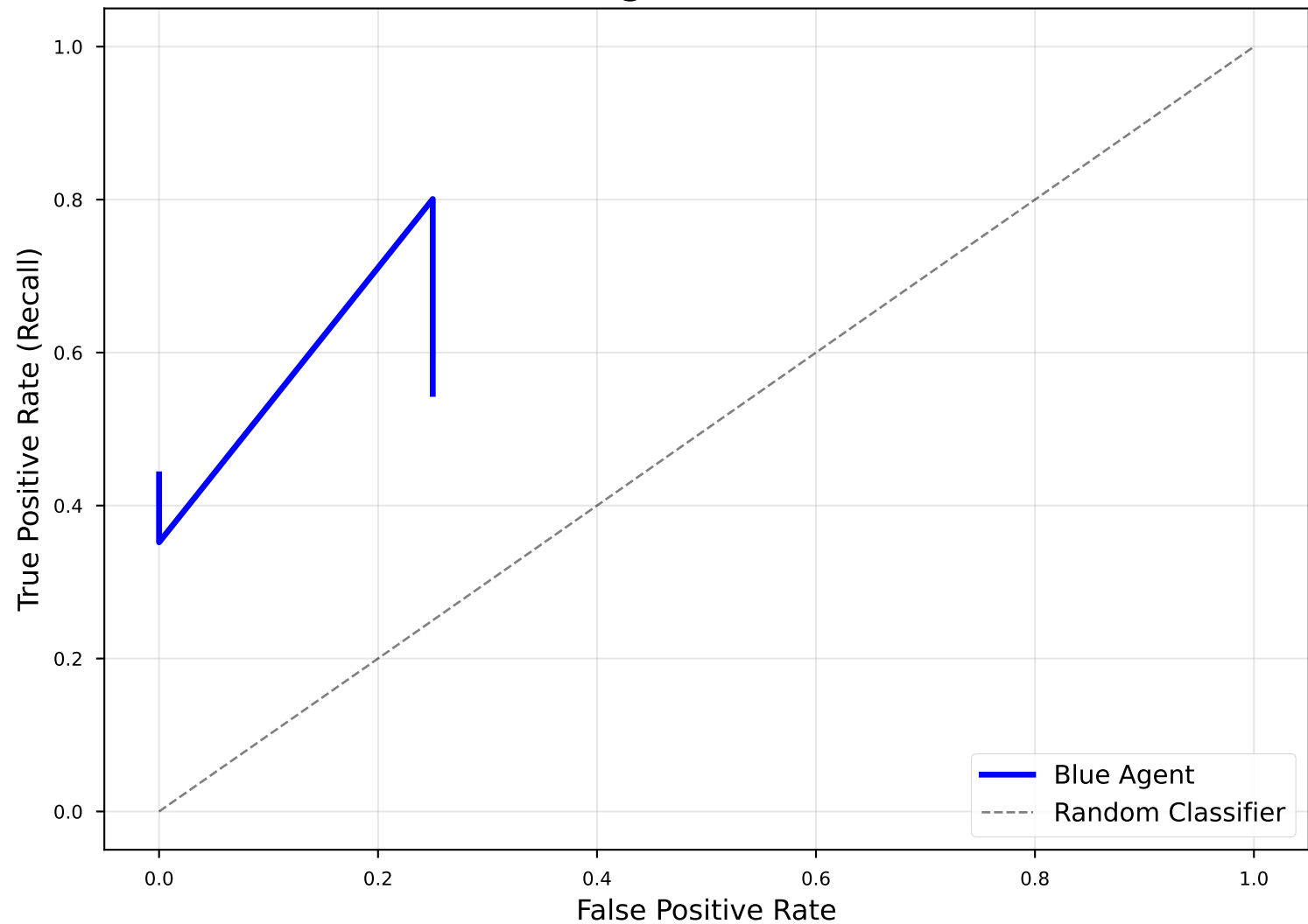
Blue Agent ROC Curve
