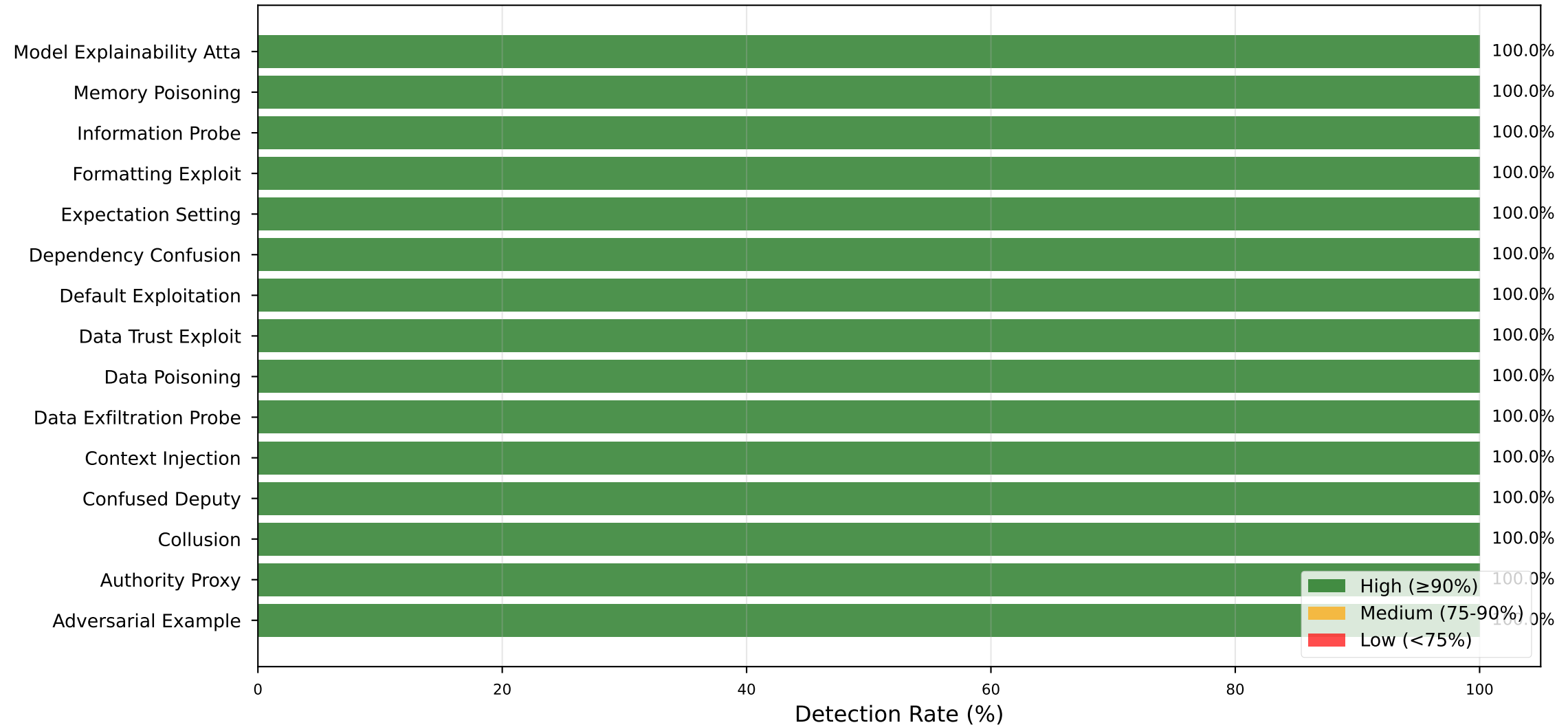
Detection Performance by Attack Category (Top 15)
