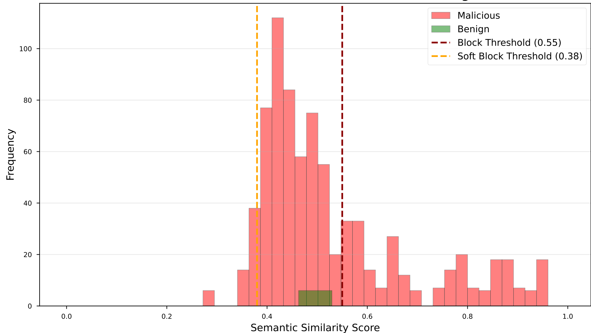
Semantic Score Distribution: Malicious vs Benign
