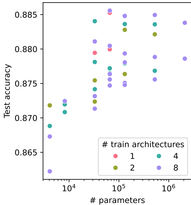
Individual train archs.
