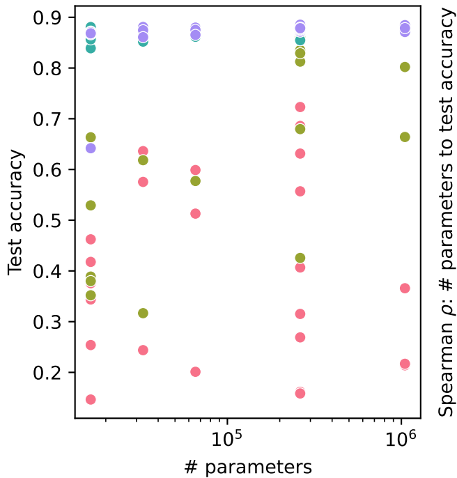
Individual val. archs.
