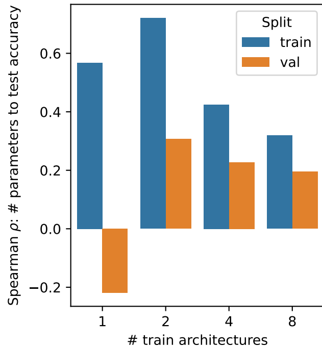
Correlations
