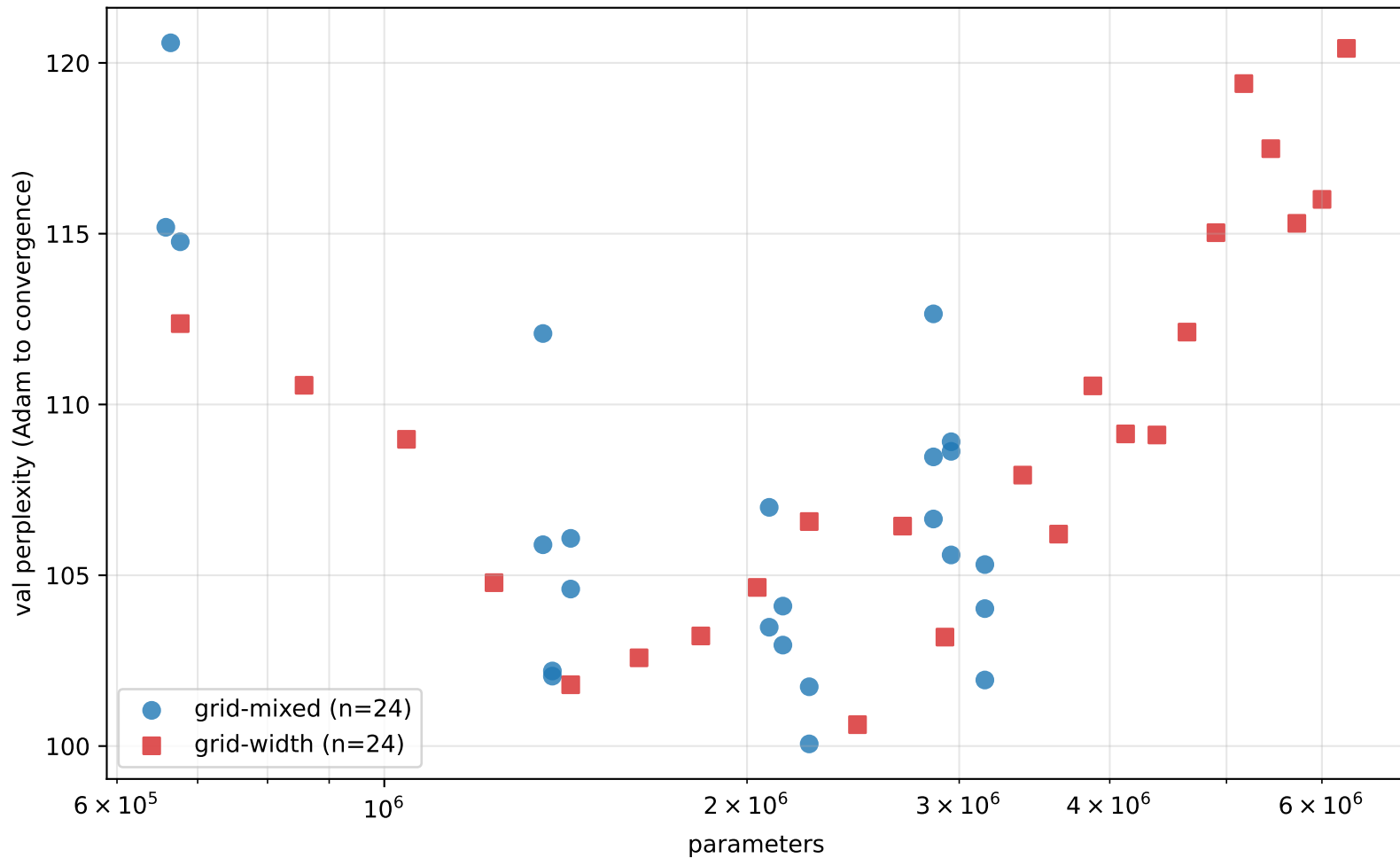
Shakespeare Adam grid baselines (3L, ctx 64) — params vs val ppl
