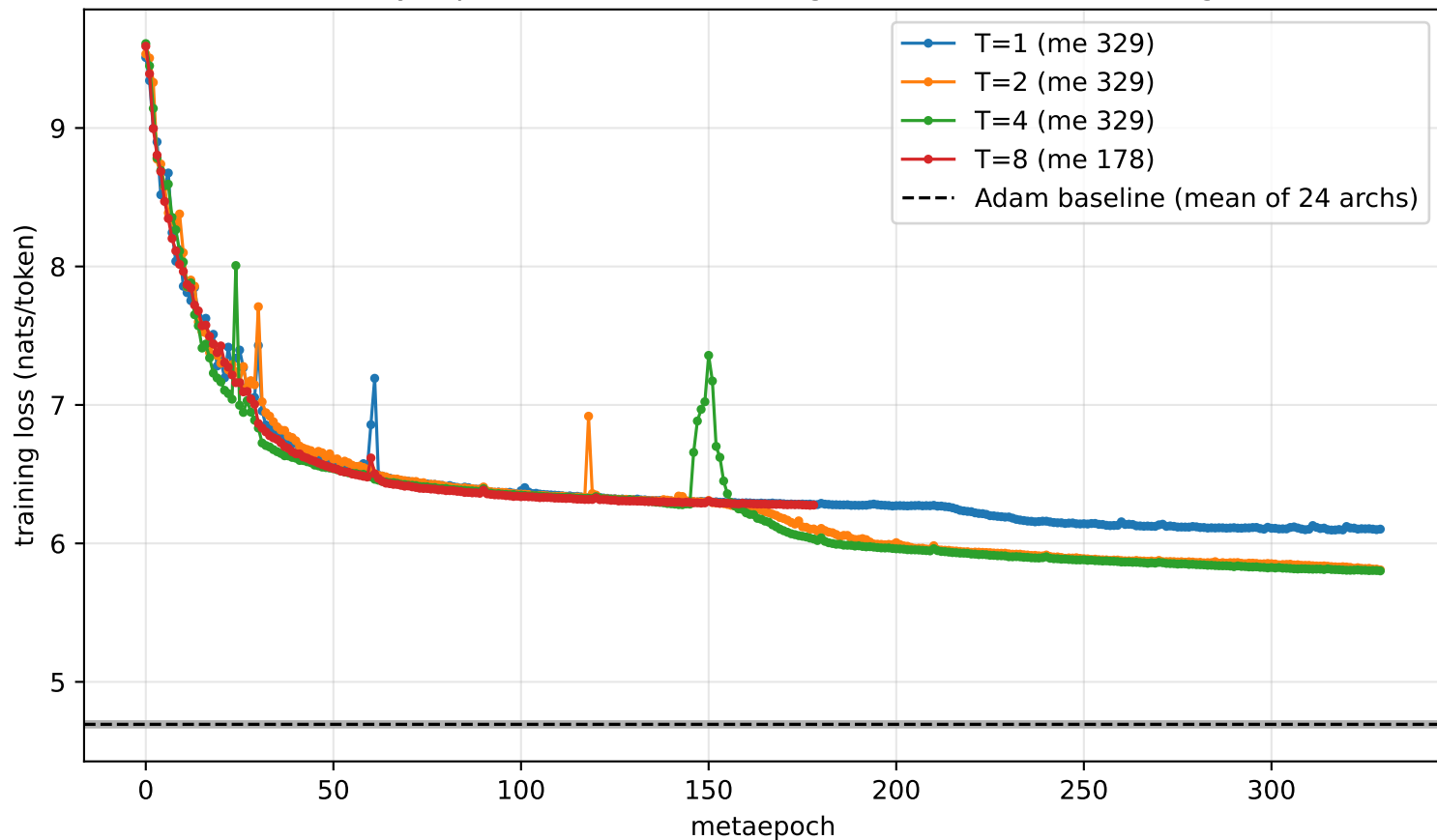
width study rep 0 ( \text{lr}=3\text{e-}4 ) — training loss vs Adam-to-convergence
