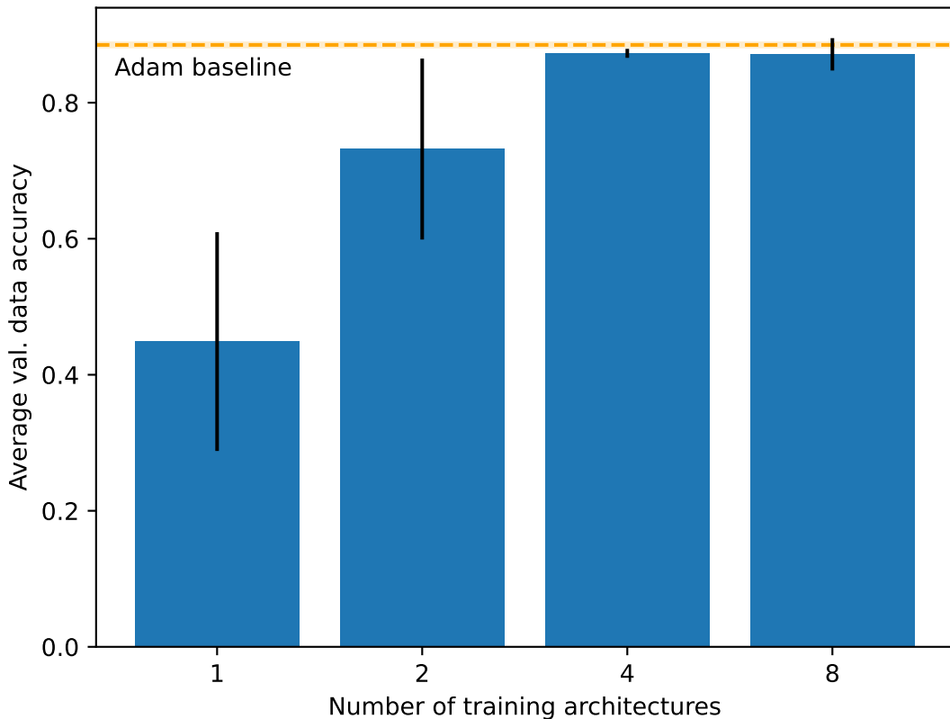
FashionMNIST heldout architecture performance
