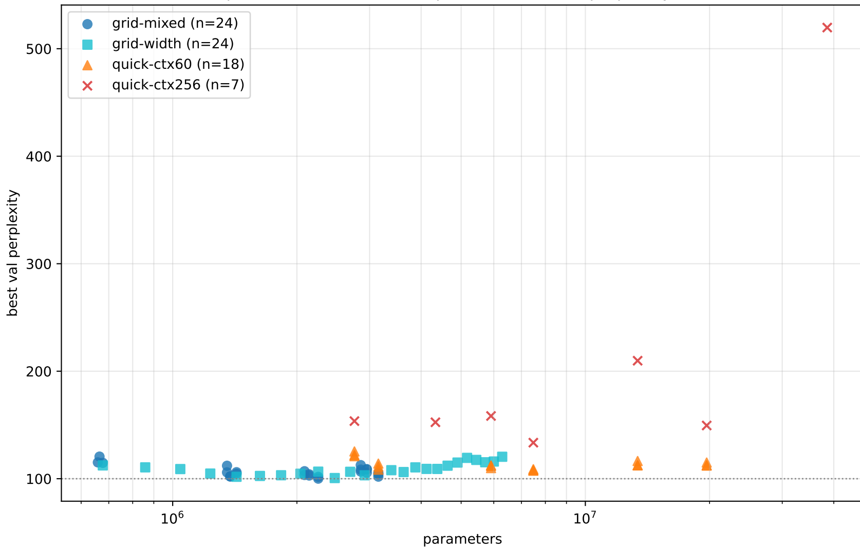
Shakespeare Adam baselines — parameters vs val perplexity (10k BPE)
