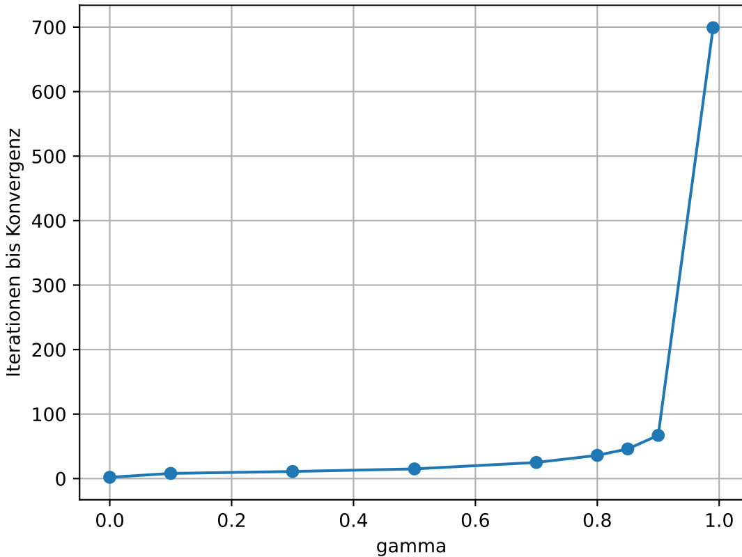
gamma vs. Iterationen (theta=0.00001)
