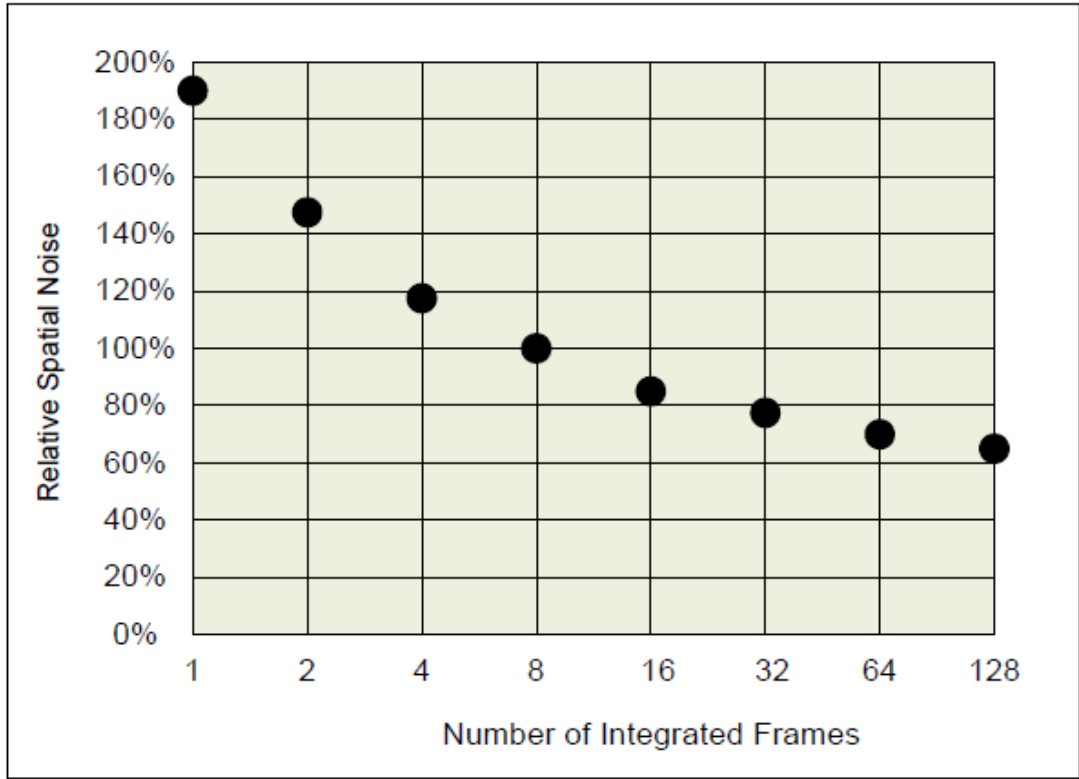
Figure 9 - Relative Spatial Noise after FFC vs. Number of Integrated Frames ((defaults is 8)
