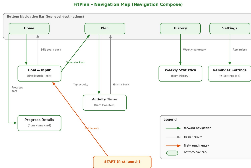
Figure 6 – Navigation map of Compose screens
