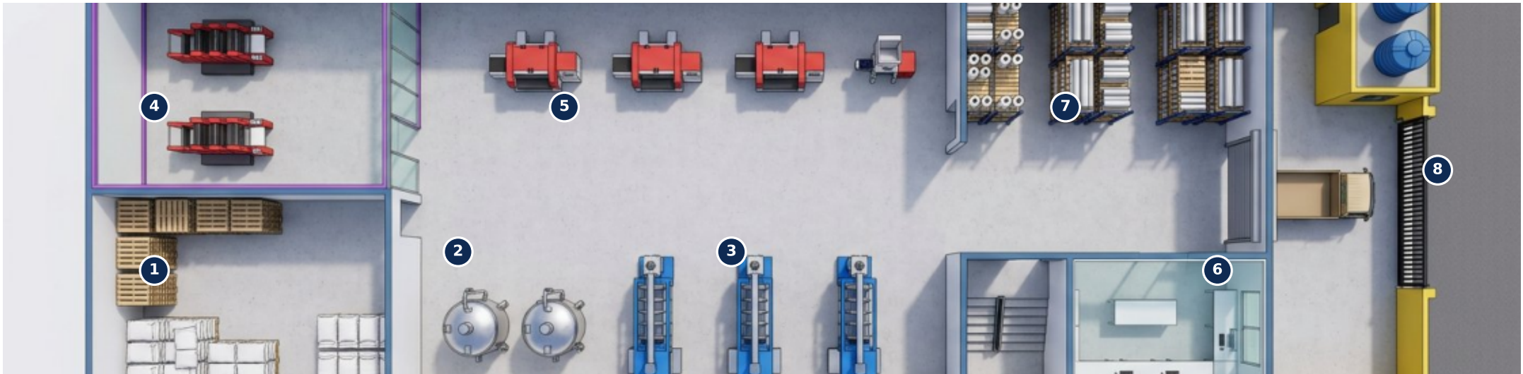
GROUND FLOOR PLAN (Production hall 39.40 × 10.17m — N on left)
