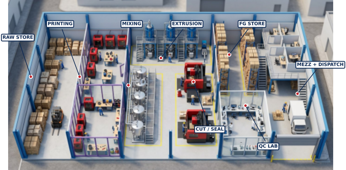
3D CUTAWAY VIEW (without roof)
