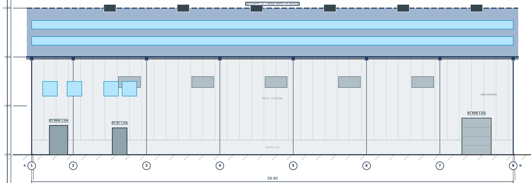
LEFT / WEST ELEVATION (from driveway — 4.0m setback)
