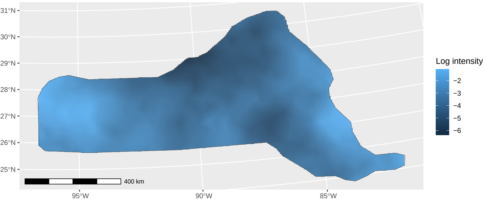
A realisation of the true underlying log intensity
