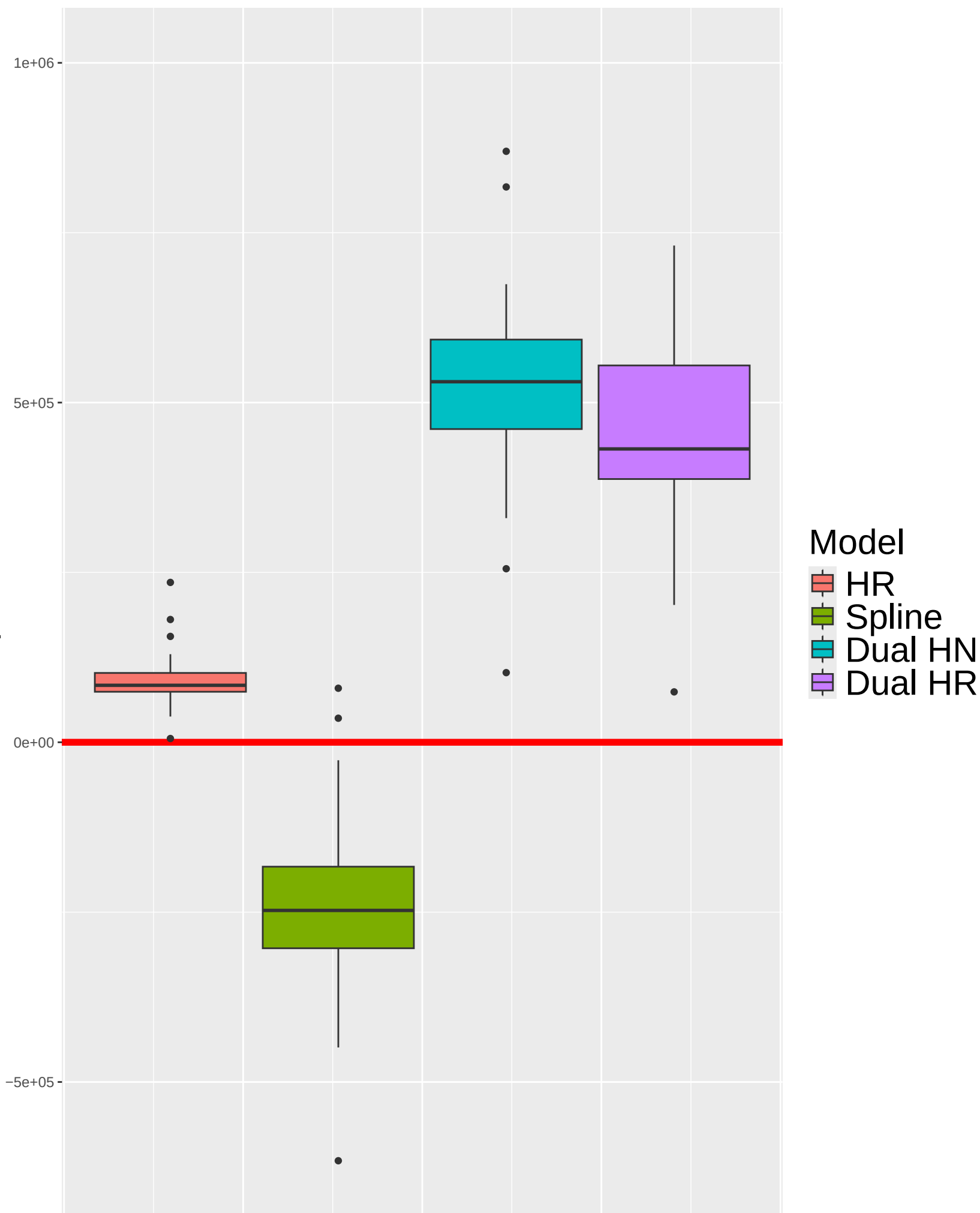
Integrated Squared Error on mean log lambda
