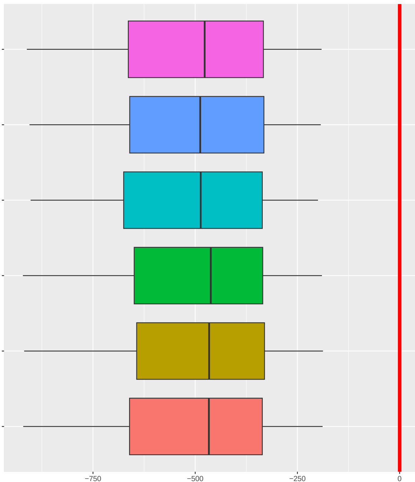
Integrated Absolute Error on median intensity
