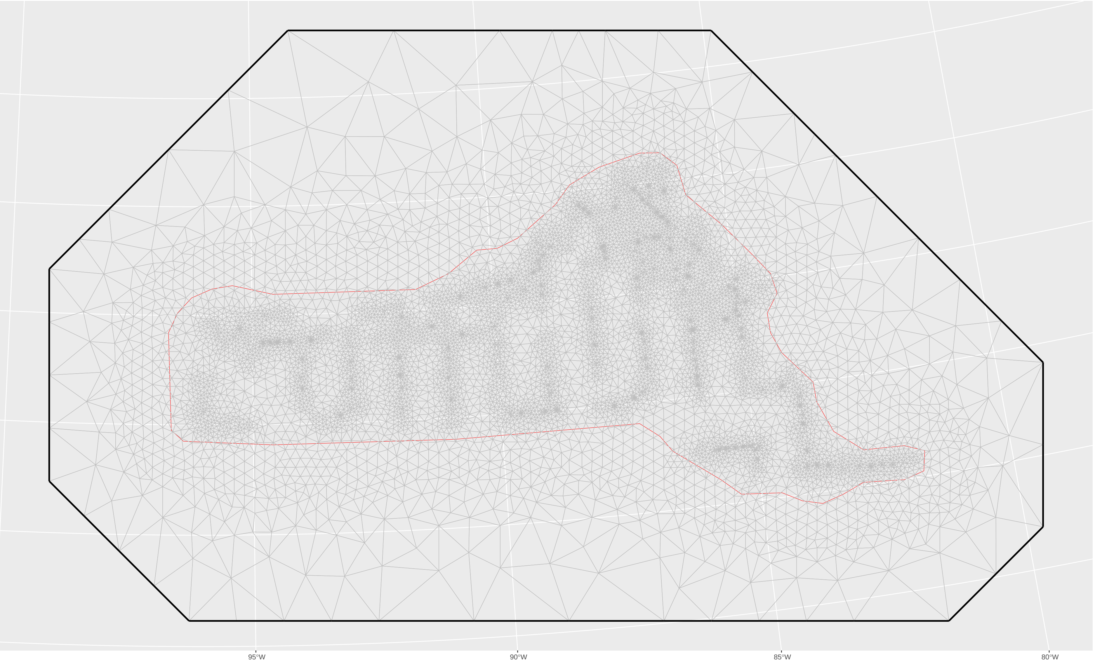
A mesh with spatially varying edge lengths
