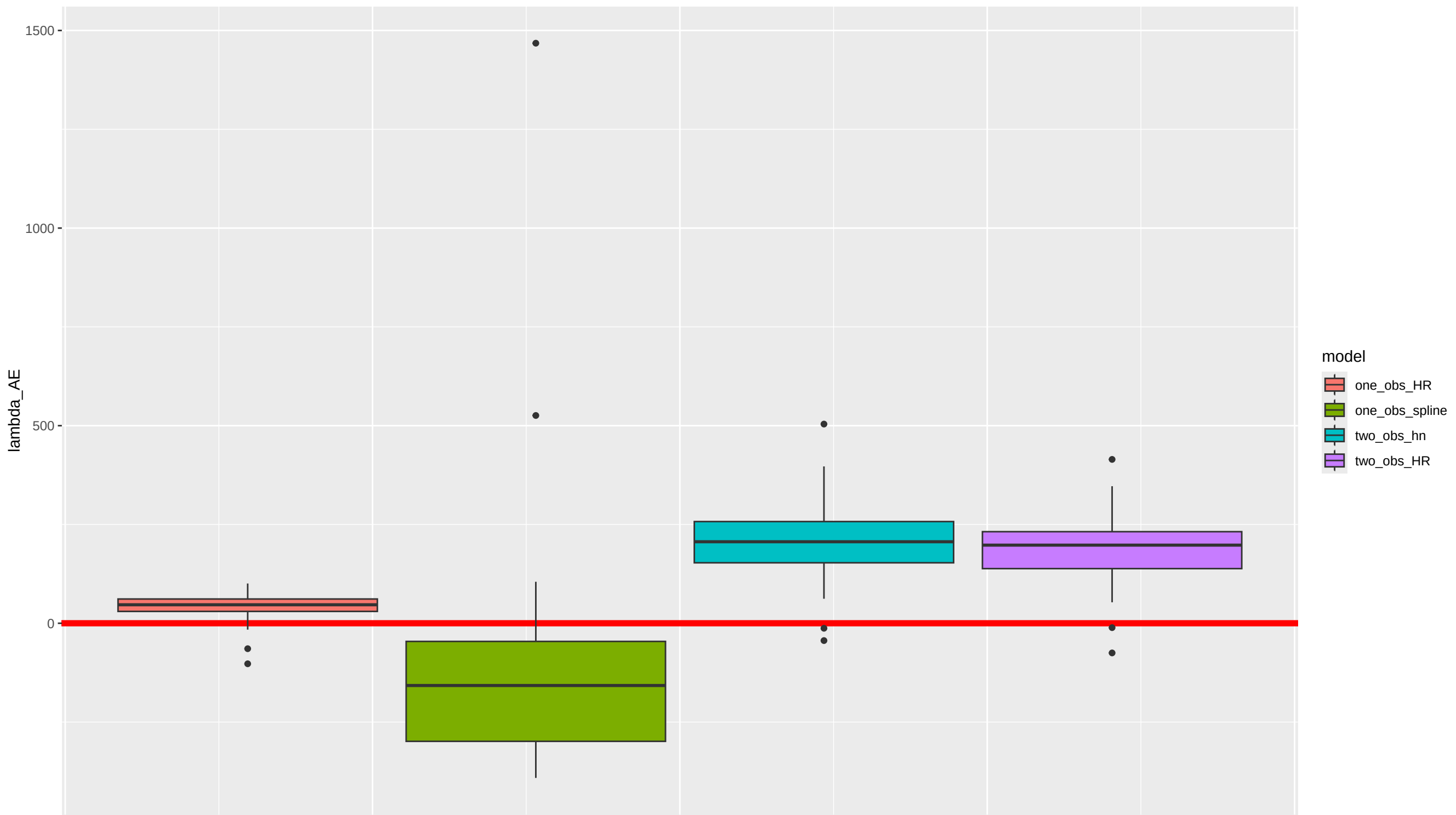
integrated AE on median lambda
