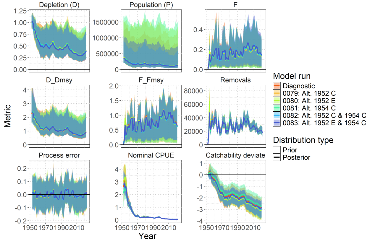
Figure 22: One-off sensitivity group: Early data . Posterior time series distributions for key derived quantities over time (line = median, shading = 95% credible interval): depletion (D), absolute population size in numbers (P), fishing mortality (F), stock status relative to MSY reference points ( D/D_{MSY} , F/F_{MSY} ), total removals in numbers, process error, nominal CPUE (numbers caught per 1000 hooks), and catchability deviates. The diagnostic model (0100) is shown in orange.
