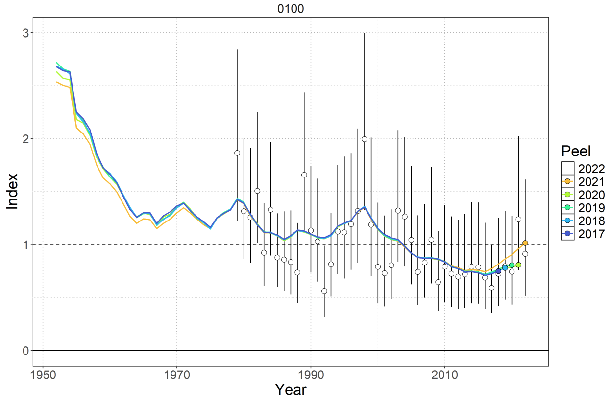
Figure 11: Standardized indices of relative abundance used in the diagnostic case model ( 0100 ). Open circles show observed values (standardized to mean of 1; black horizontal line) and the vertical bars indicate the observation error (95% confidence interval). One year ahead ‘model-free’ hindcast predictions are shown by the colored lines, where the color indicates the last year of index data seen by the model. The predicted value is shown one year-ahead with the colored point.
