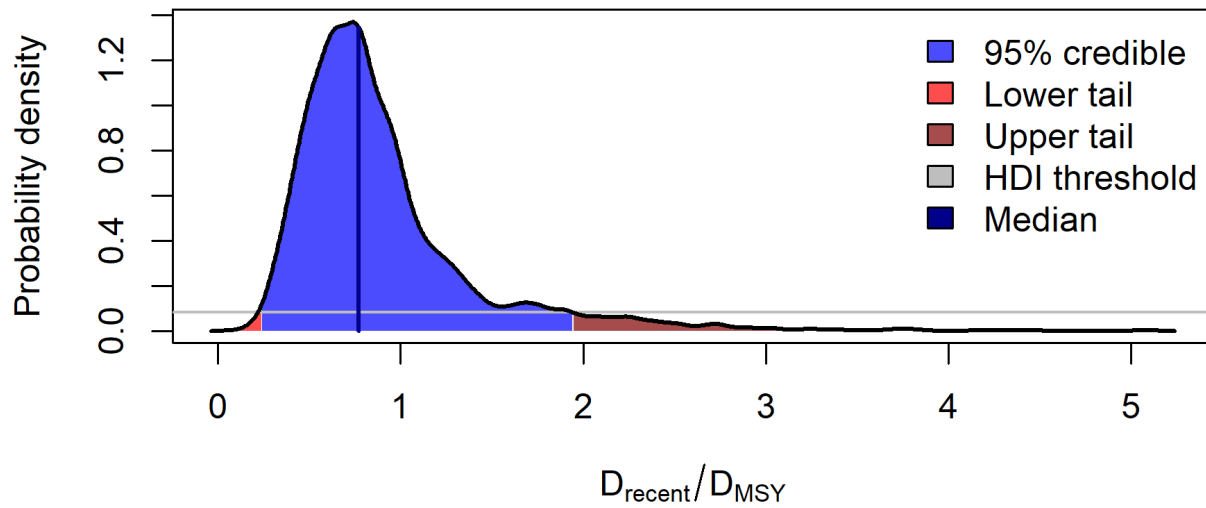
Figure 51: Comparison of equal-tailed intervals (ETI) and highest density intervals (HDI) for the posterior distribution of recent depletion relative to MSY ( D_{\text{recent}}/D_{\text{MSY}} ). Panel A shows the 95% ETI with equal probability (2.5%) in each tail. Panel B shows the 95% HDI, which contains the most probable values and is bounded by the horizontal threshold line (gray) where all values above have higher probability density than values below.
