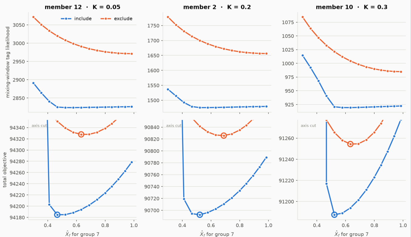
Fixed-parameter profile against the reporting rate (group 7) — rings mark each arm's argmin
