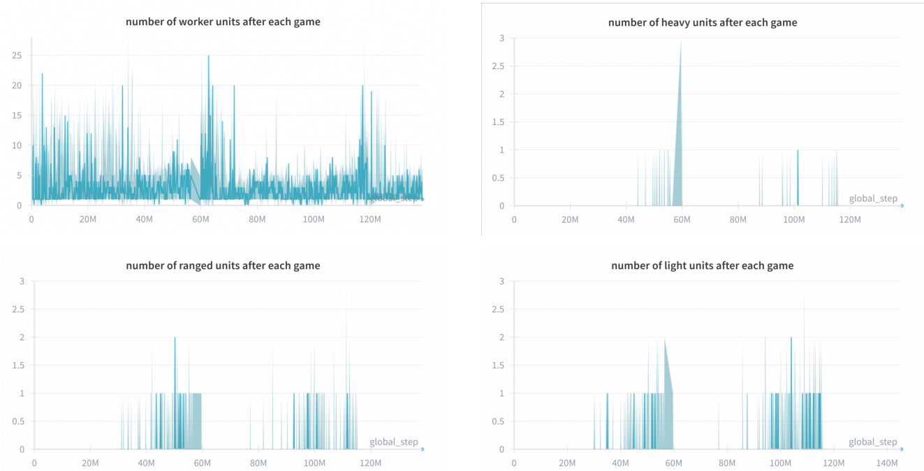
Figure 4. Number of units after each game for the agents initialized with worker focused (shown are 2 full reset cycles).
