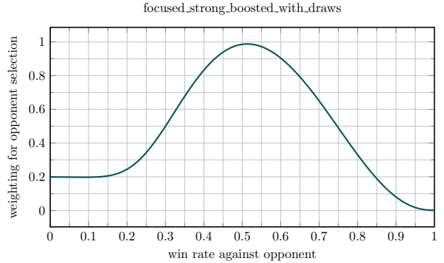
Figure 4. Prioritization function for the Exploiters in PFSP.
