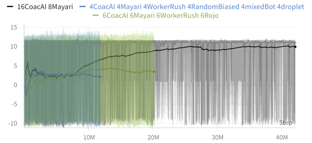
Figure 6. Episode rewards (y-axis) as a function of training timesteps (x-axis) on the BC-FT agent.
