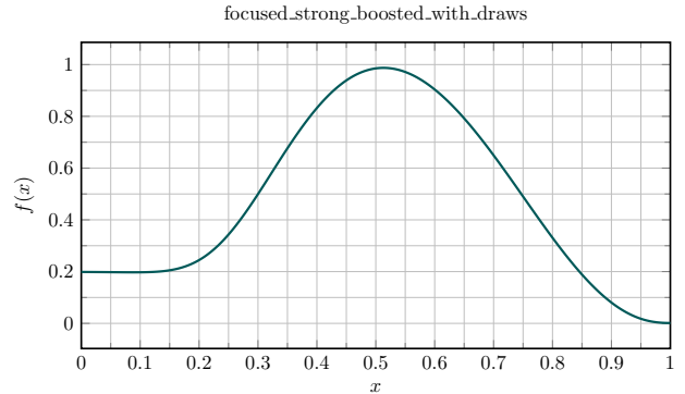
Figure 4. Prioritization function for the Exploiters in PFSP.
