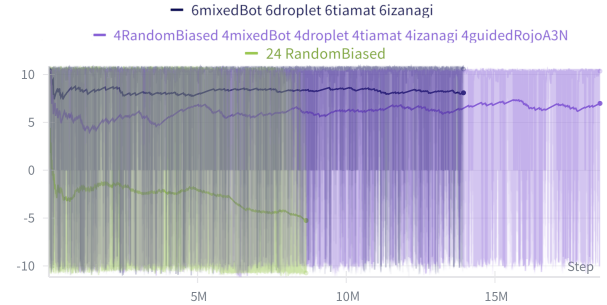
Figure 7. Episode rewards (y-axis) as a function of training timesteps (x-axis) on the final agent.
