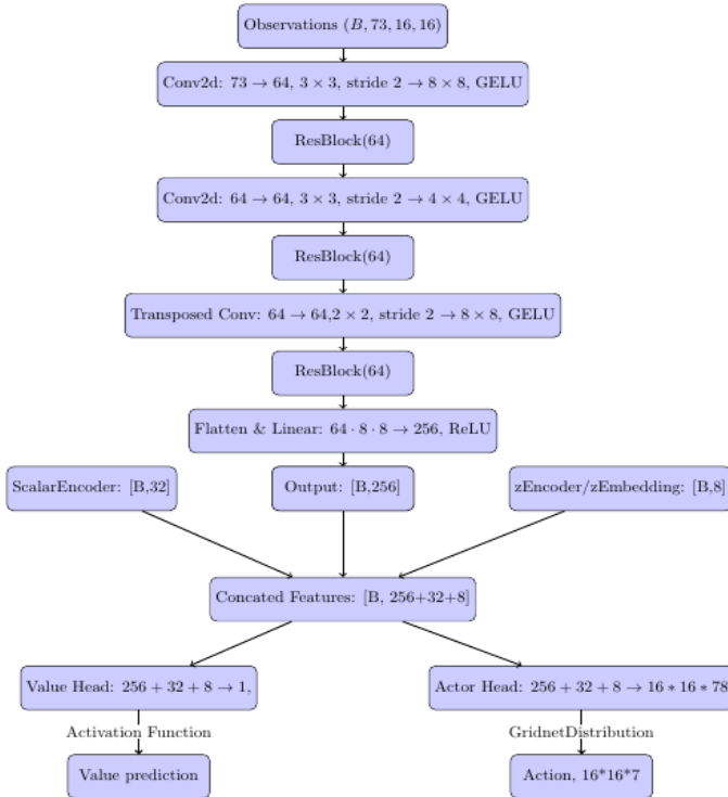
Figure 5. The Network Architecture
