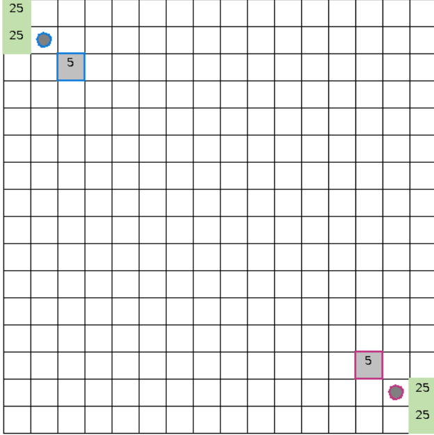
Figure 1. Screenshot of the initial state of the basesWorkers16x16A map.
